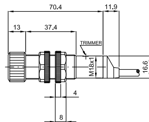
M12 CONNECTOR
